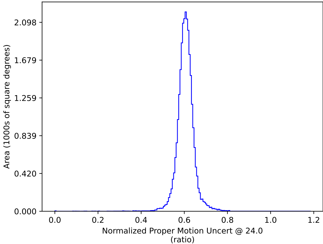
noroll_mjdp0_v3.4_10yrs : Normalized Proper Motion Uncert @ 24.0
