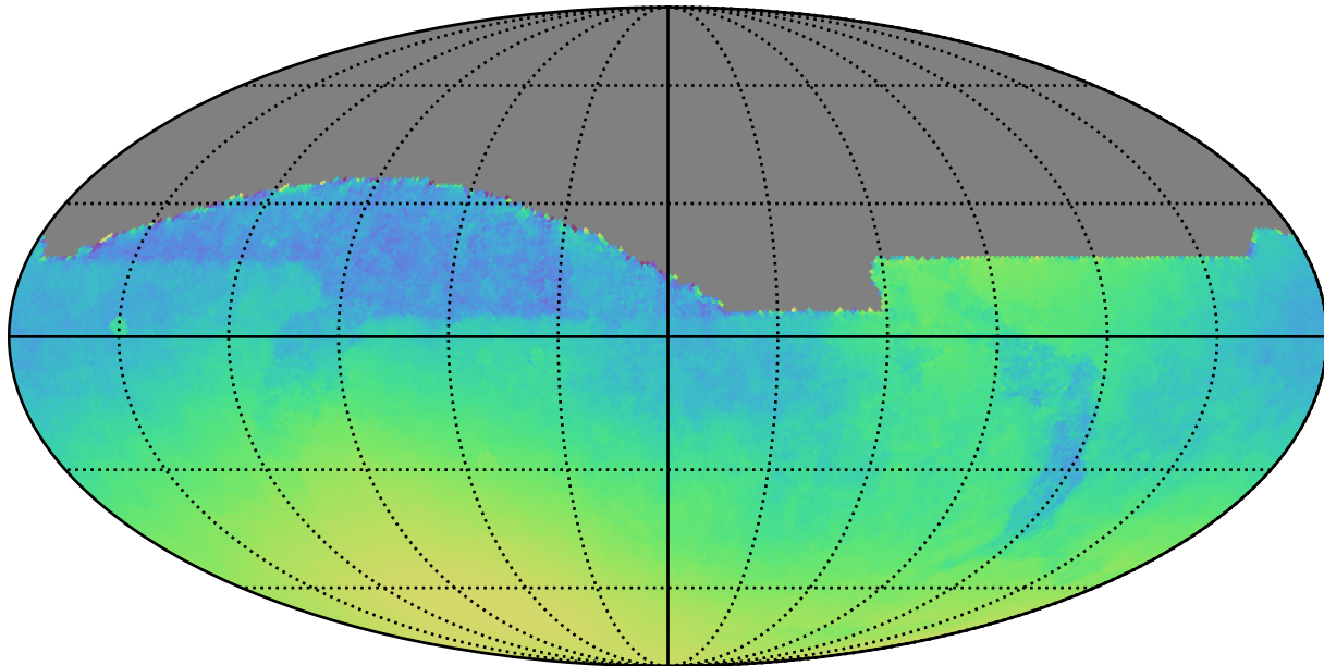
noroll_mjdp0_v3.4_10yrs : Normalized Parallax Uncert @ 24.0
