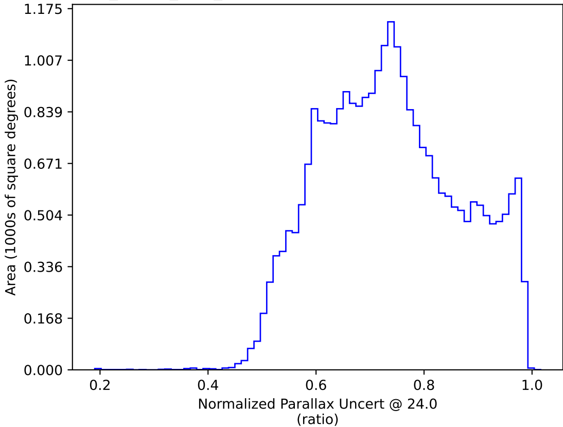
noroll_mjdp0_v3.4_10yrs : Normalized Parallax Uncert @ 24.0
