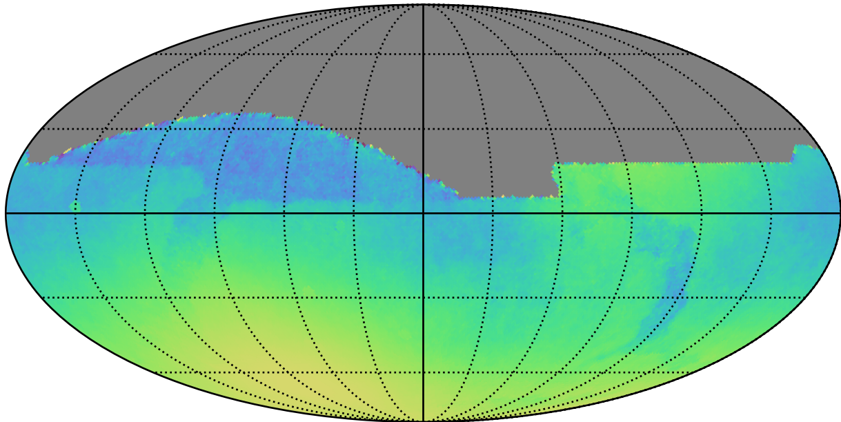
noroll_mjdp0_v3.4_10yrs : Normalized Parallax Uncert @ 22.4
