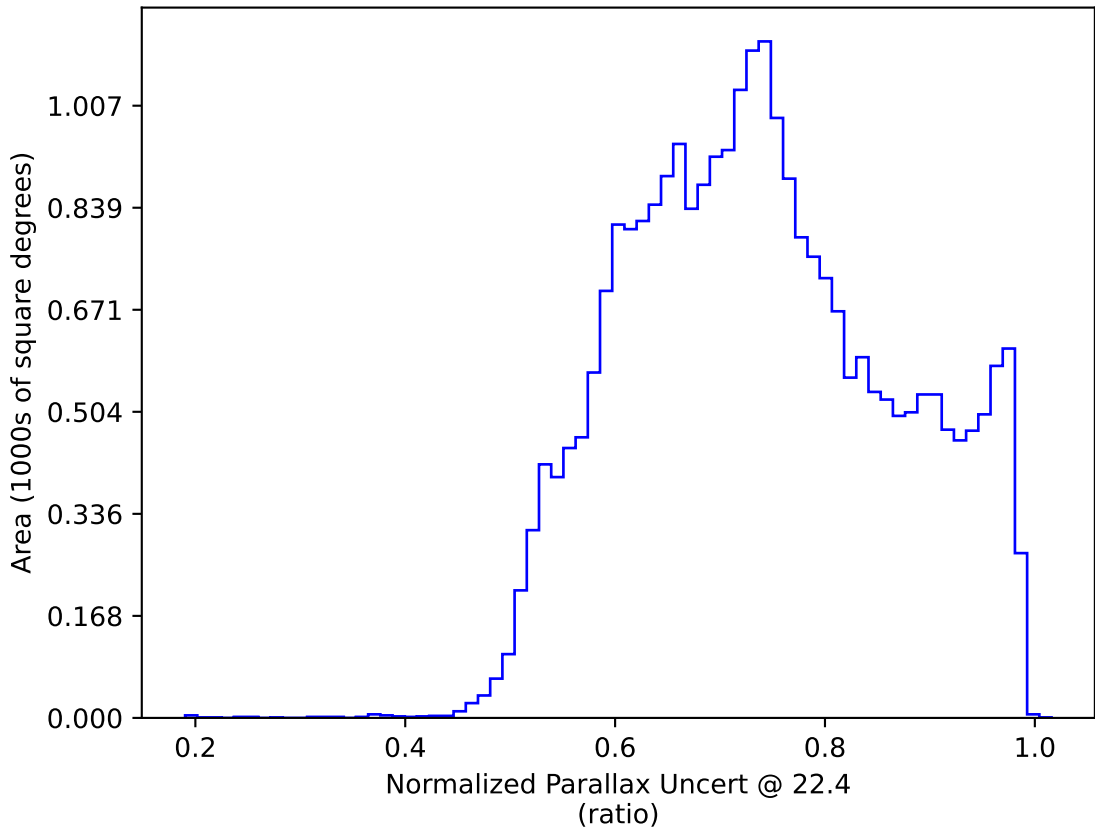
noroll_mjdp0_v3.4_10yrs : Normalized Parallax Uncert @ 22.4
