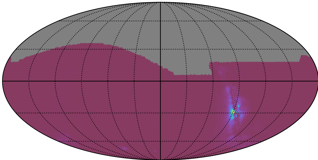
noroll_mjdp0_v3.4_10yrs : NlcPoints
