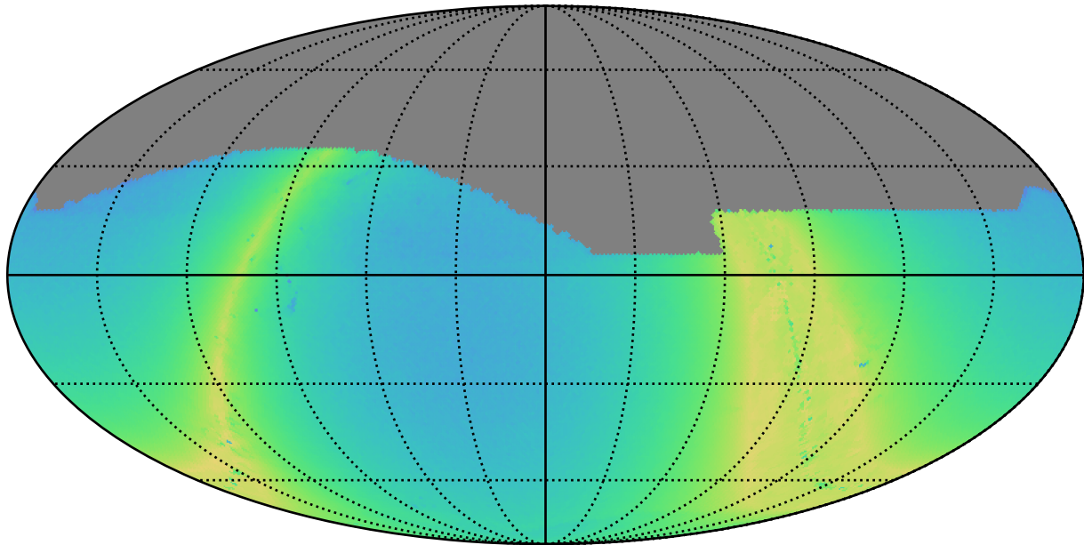
noroll_mjdp0_v3.4_10yrs z: N stars to Precision 0.20
