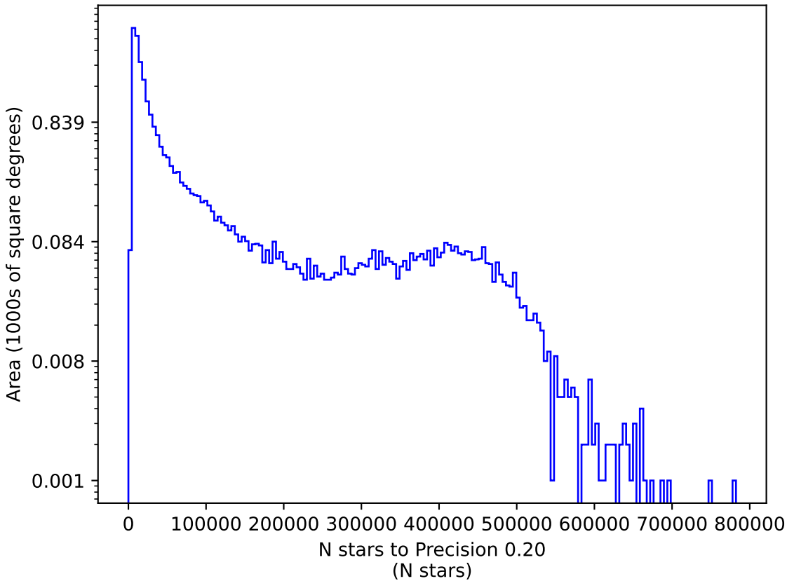
noroll_mjdp0_v3.4_10yrs r: N stars to Precision 0.20
