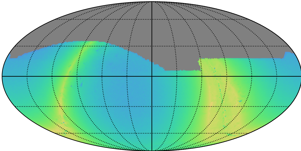
noroll_mjdp0_v3.4_10yrs i: N stars to Precision 0.20
