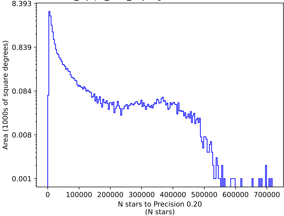
noroll_mjdp0_v3.4_10yrs g: N stars to Precision 0.20
