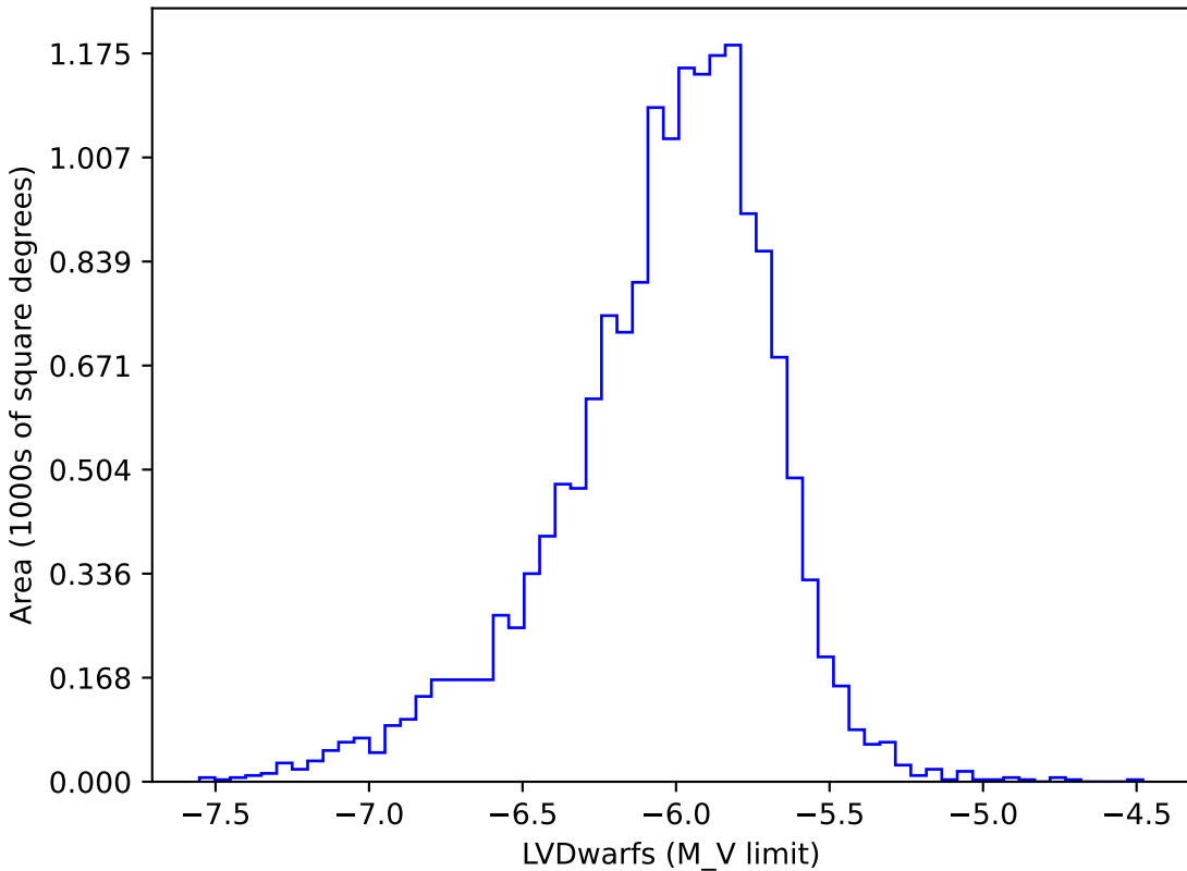
noroll_mjdp0_v3.4_10yrs gi: LVDwarfs
