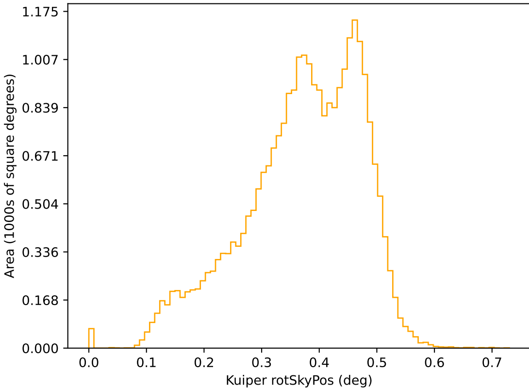
noroll_mjdp0_v3.4_10yrs r: Kuiper rotSkyPos
