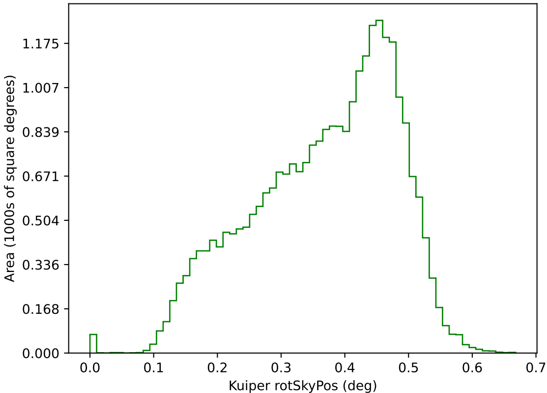
noroll_mjdp0_v3.4_10yrs g: Kuiper rotSkyPos
