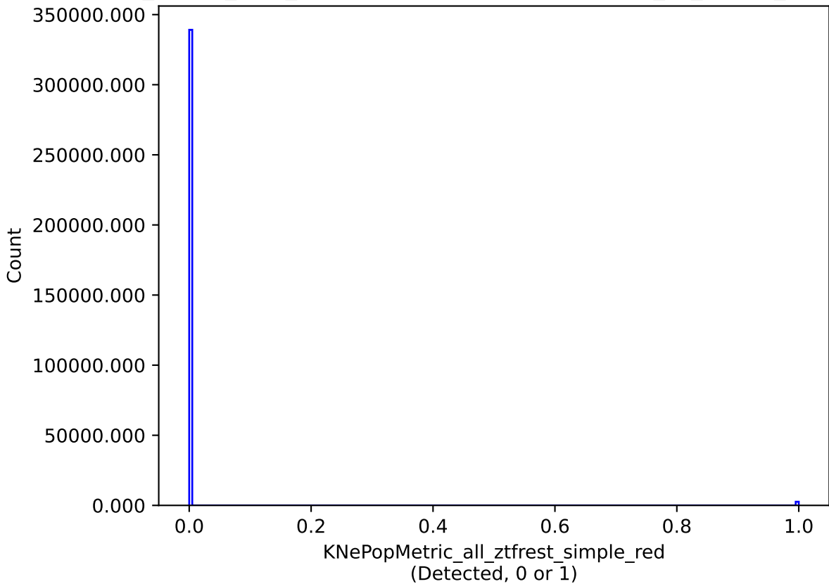
noroll_mjdp0_v3.4_10yrs all models: KNePopMetric_all_ztfrest_simple_red
