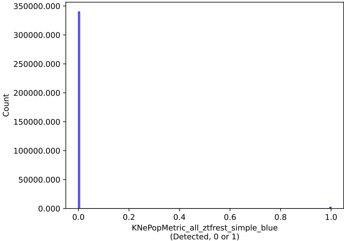
noroll_mjdp0_v3.4_10yrs all models: KNePopMetric_all_ztfrest_simple_blue
