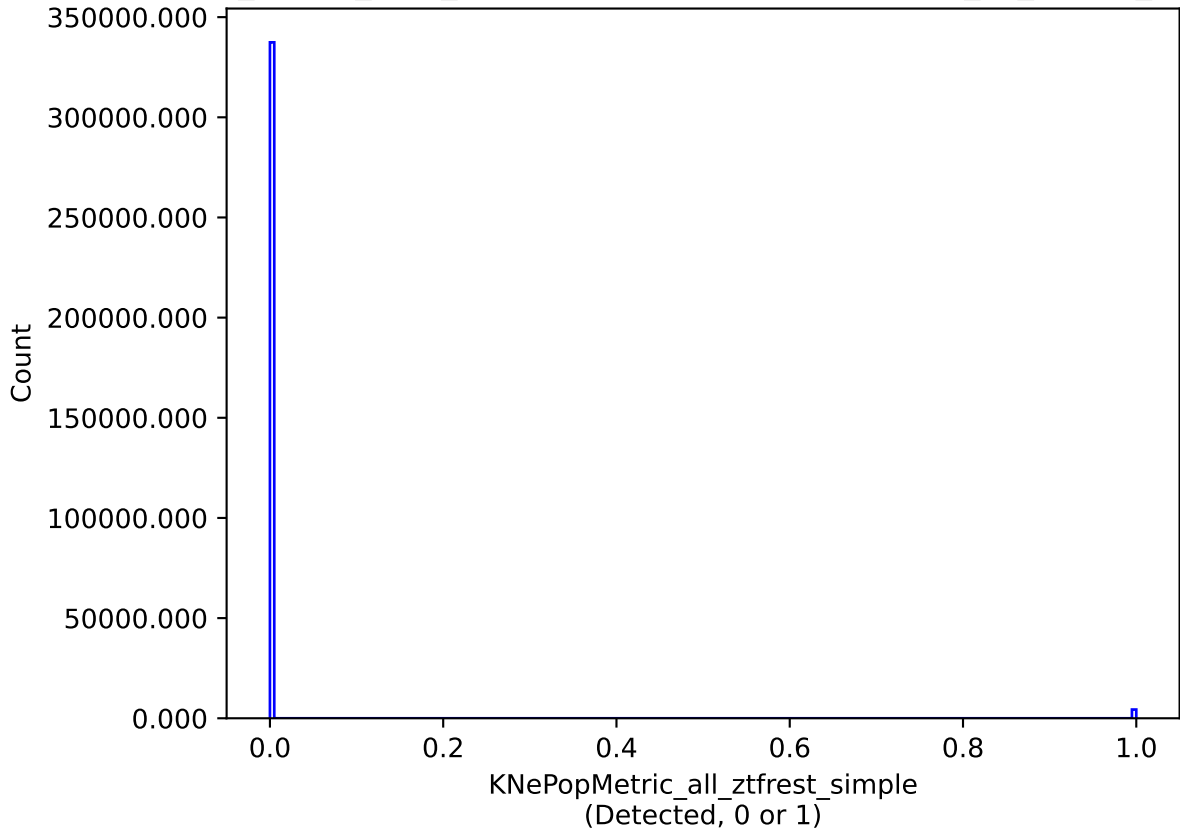
noroll_mjdp0_v3.4_10yrs all models: KNePopMetric_all_ztfrest_simple
