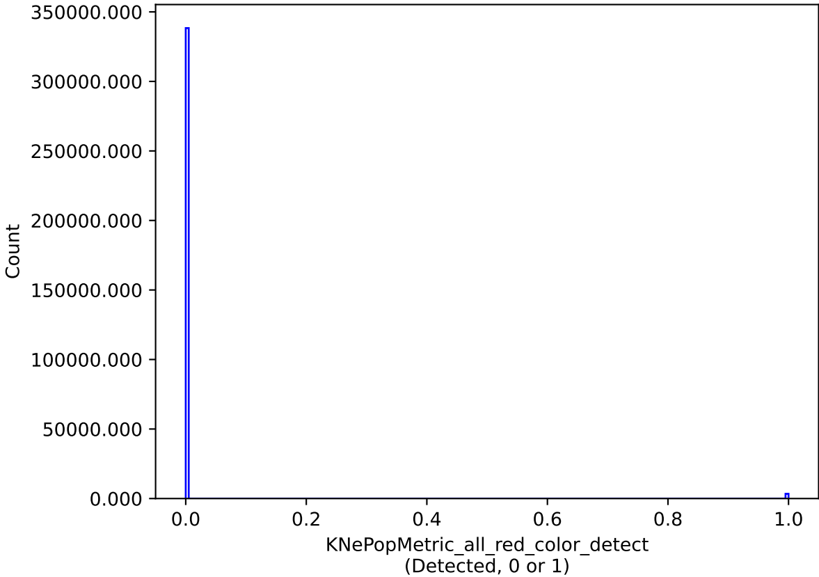
noroll_mjdp0_v3.4_10yrs all models: KNePopMetric_all_red_color_detect
