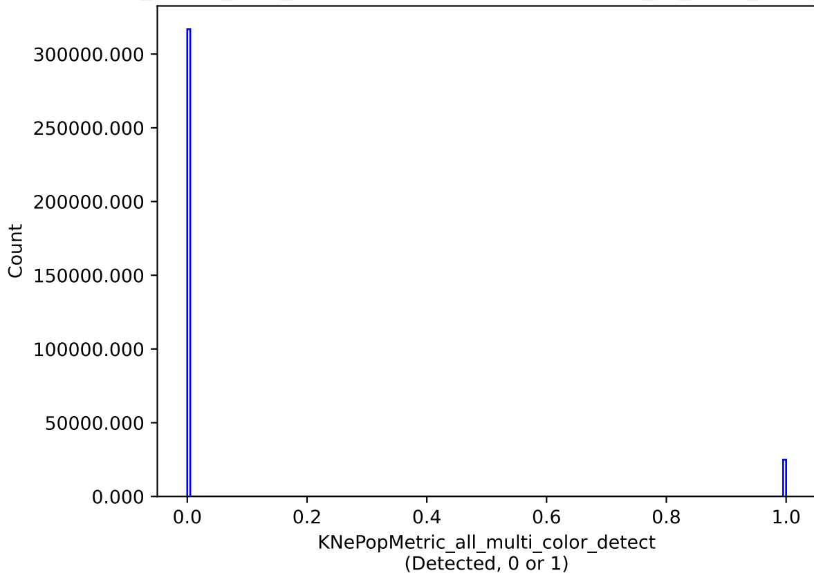
noroll_mjdp0_v3.4_10yrs all models: KNePopMetric_all_multi_color_detect
