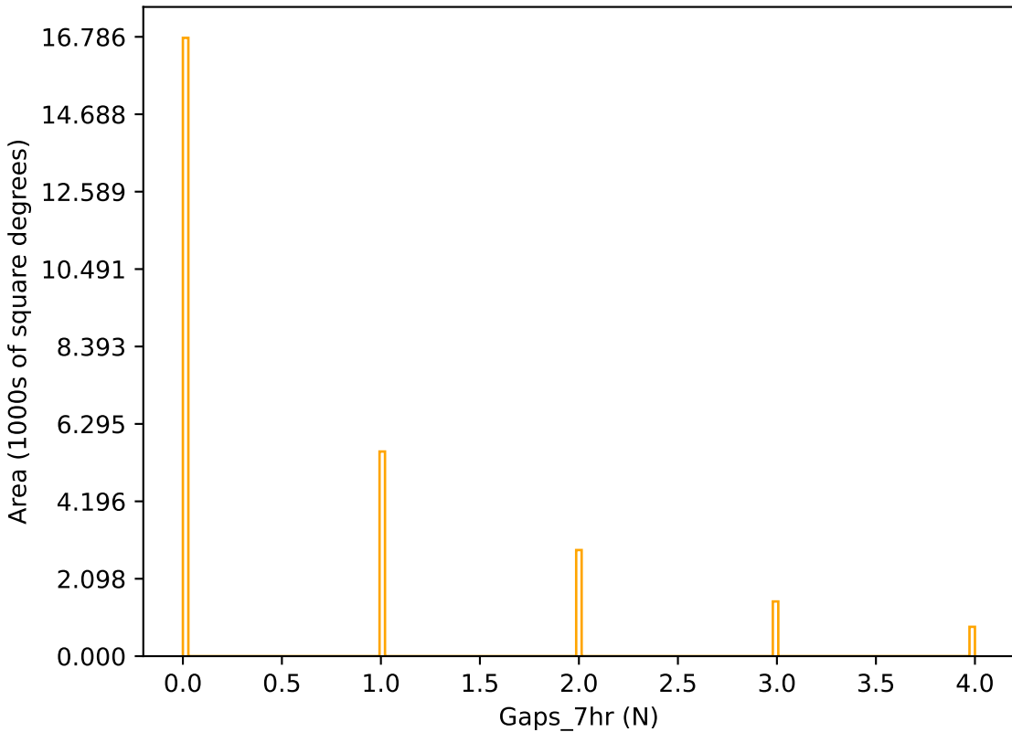
noroll_mjdp0_v3.4_10yrs r band: Gaps_7hr
