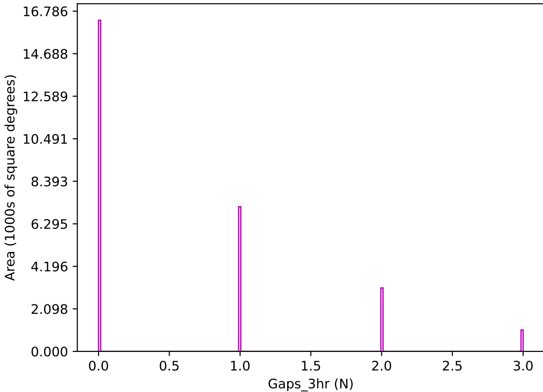
noroll_mjdp0_v3.4_10yrs z band: Gaps_3hr
