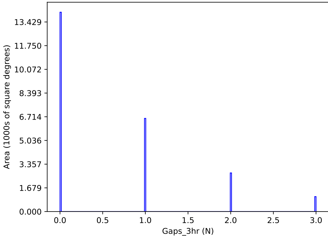
noroll_mjdp0_v3.4_10yrs y band: Gaps_3hr
