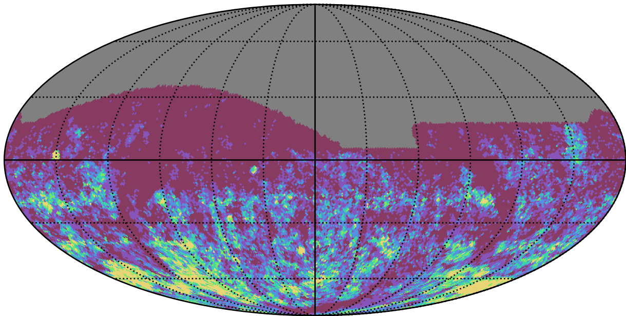
noroll_mjdp0_v3.4_10yrs r band: Gaps_3hr
