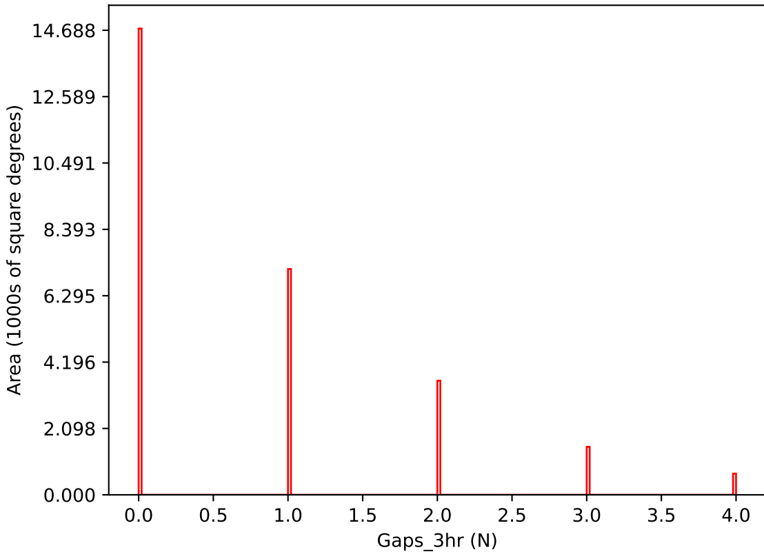
noroll_mjdp0_v3.4_10yrs i band: Gaps_3hr
