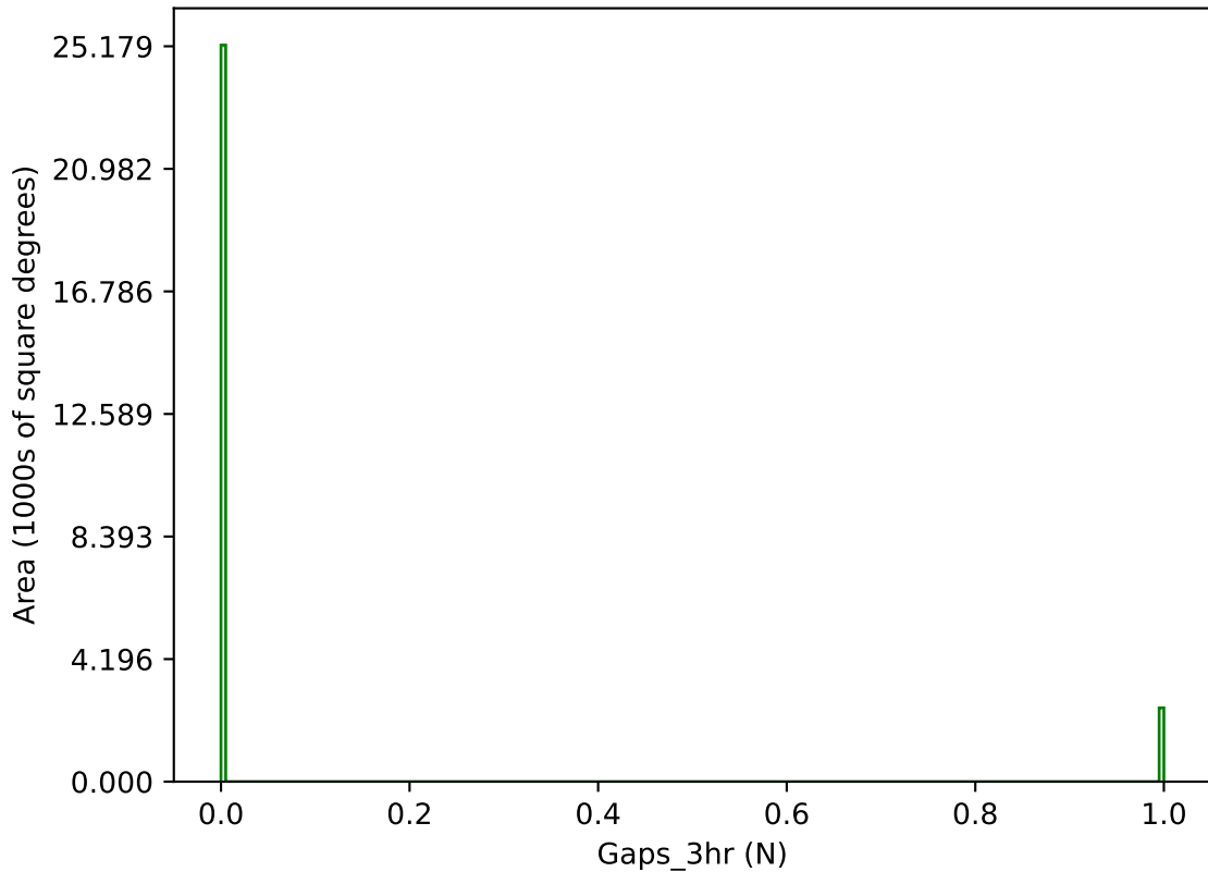
noroll_mjdp0_v3.4_10yrs g band: Gaps_3hr
