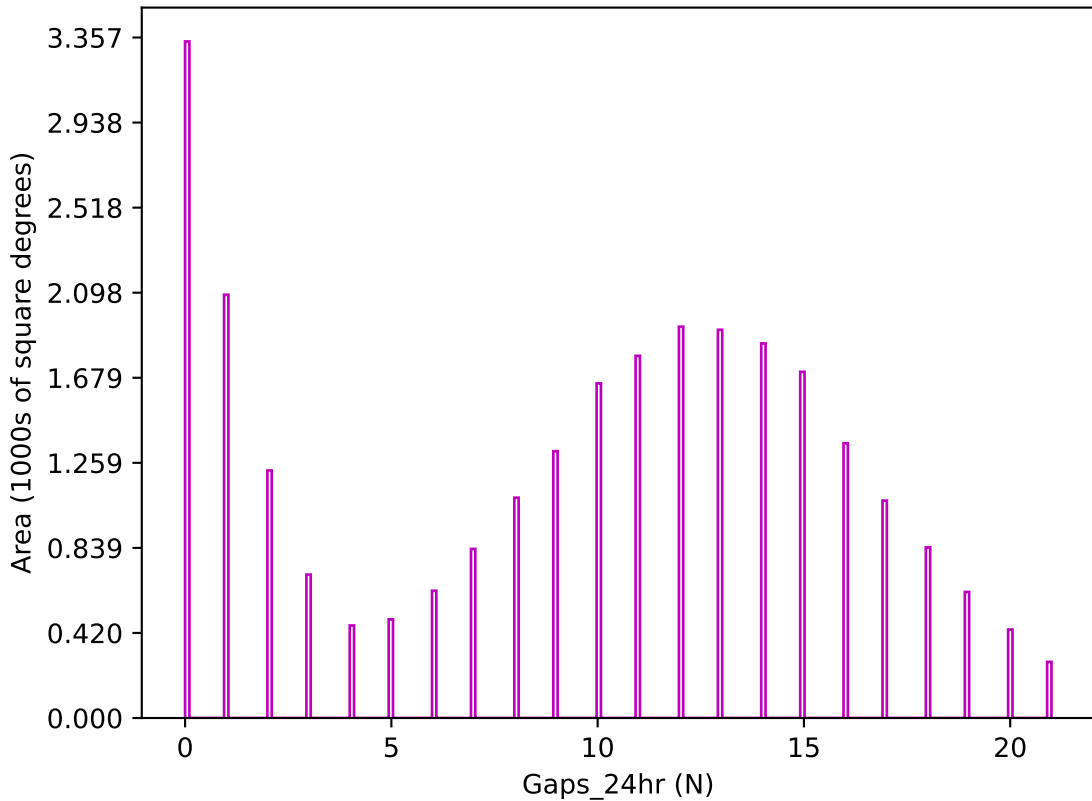
noroll_mjdp0_v3.4_10yrs z band: Gaps_24hr
