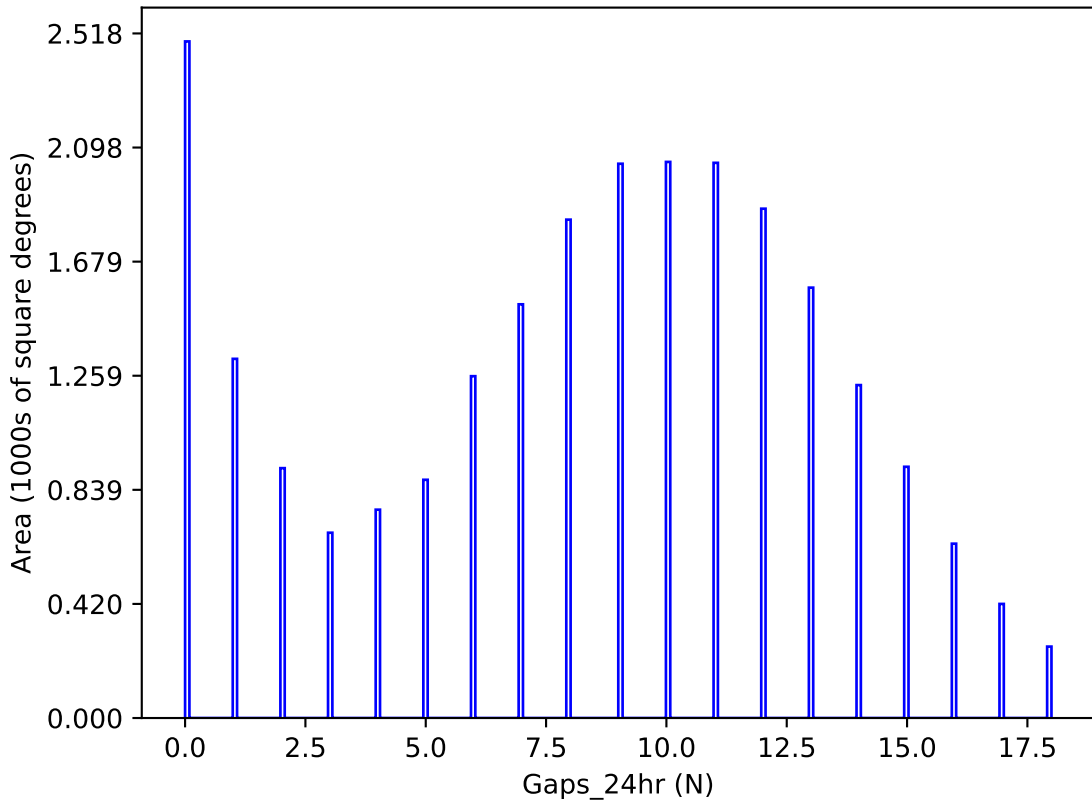
noroll_mjdp0_v3.4_10yrs y band: Gaps_24hr
