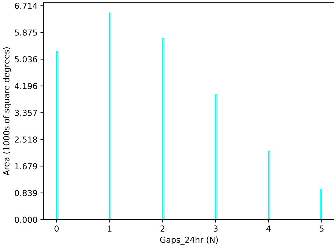
noroll_mjdp0_v3.4_10yrs u band: Gaps_24hr
