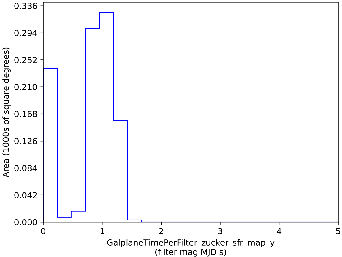
noroll_mjdp0_v3.4_10yrs : GalplaneTimePerFilter_zucker_sfr_map_y
