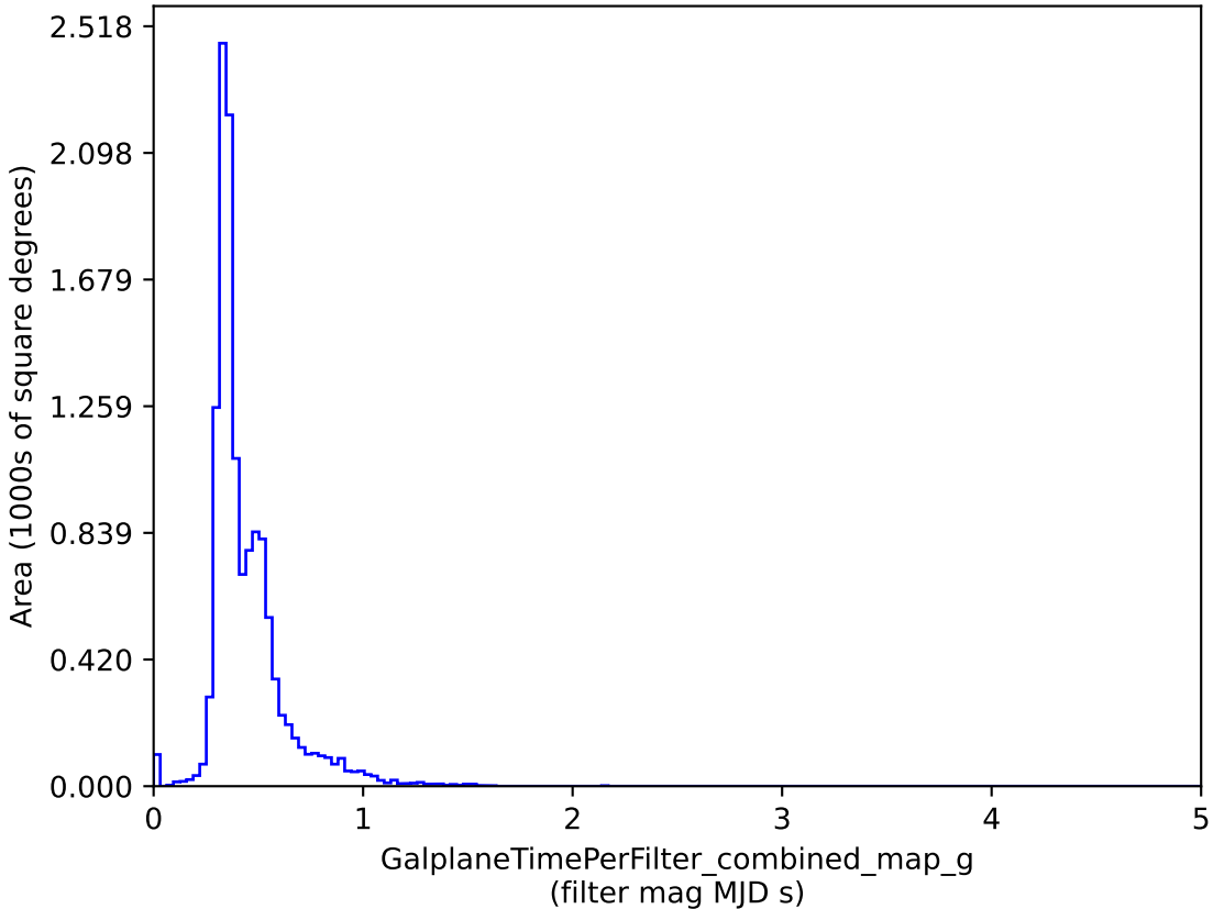
noroll_mjdp0_v3.4_10yrs : GalplaneTimePerFilter_combined_map_g
