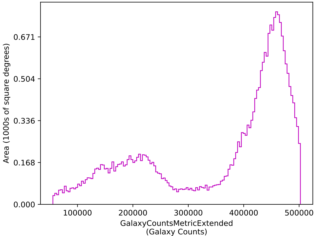
noroll_mjdp0_v3.4_10yrs z: GalaxyCountsMetricExtended
