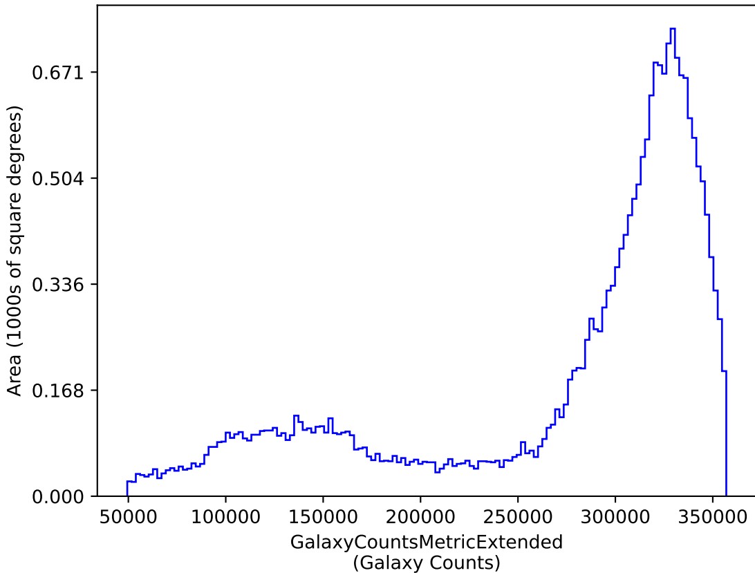
noroll_mjdp0_v3.4_10yrs y: GalaxyCountsMetricExtended
