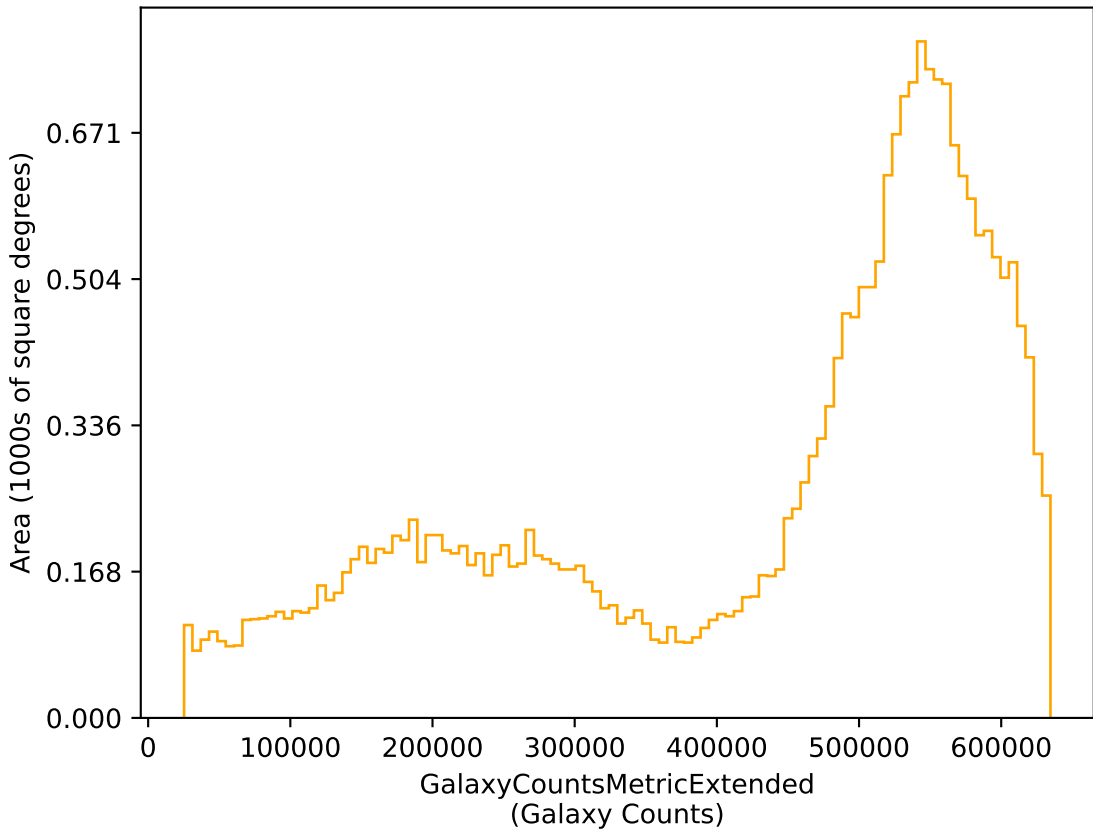
noroll_mjdp0_v3.4_10yrs r: GalaxyCountsMetricExtended
