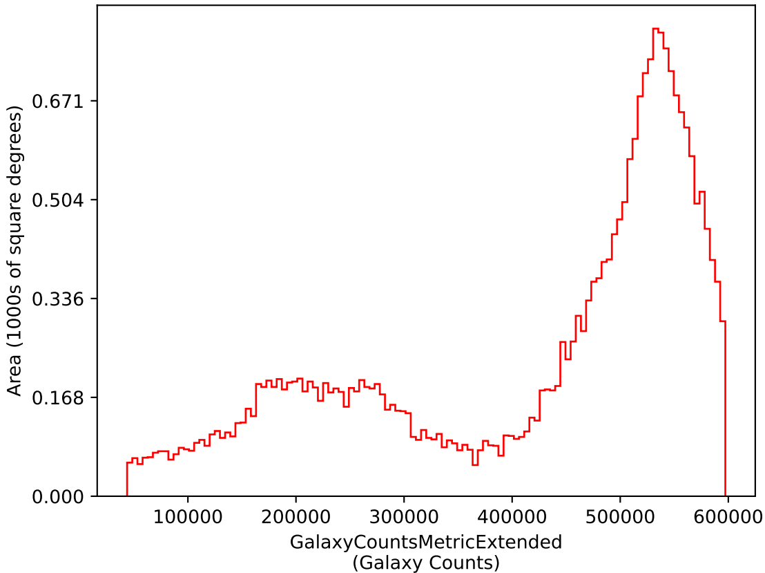
noroll_mjdp0_v3.4_10yrs i: GalaxyCountsMetricExtended
