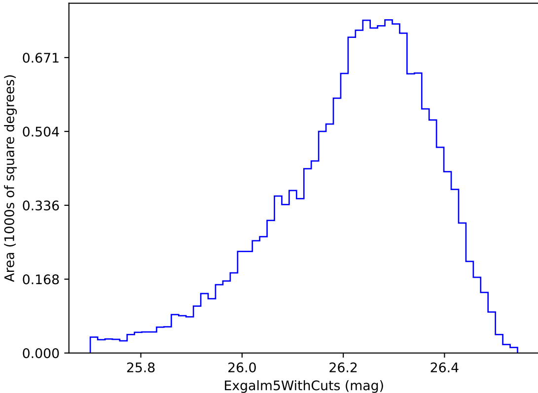
noroll_mjdp0_v3.4_10yrs i band non-DD year 7: ExgalM5WithCuts
