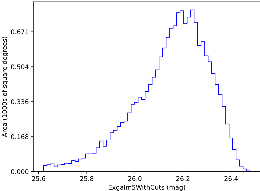
noroll_mjdp0_v3.4_10yrs i band non-DD year 6: ExgalM5WithCuts
