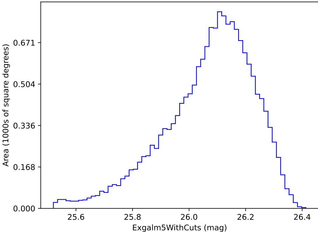
noroll_mjdp0_v3.4_10yrs i band non-DD year 5: ExgalM5WithCuts
