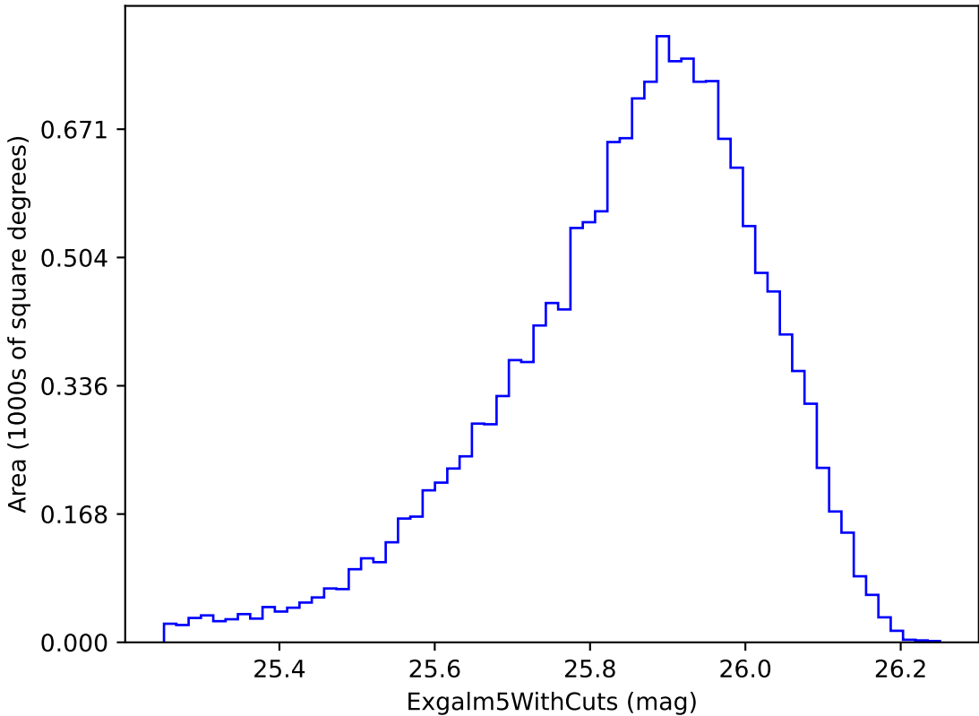
noroll_mjdp0_v3.4_10yrs i band non-DD year 3: ExgalM5WithCuts
