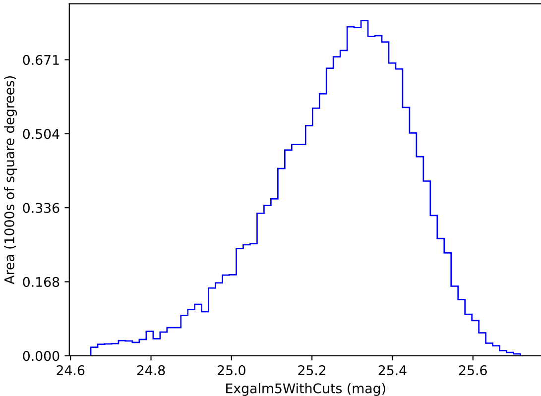
noroll_mjdp0_v3.4_10yrs i band non-DD year 1: ExgalM5WithCuts
