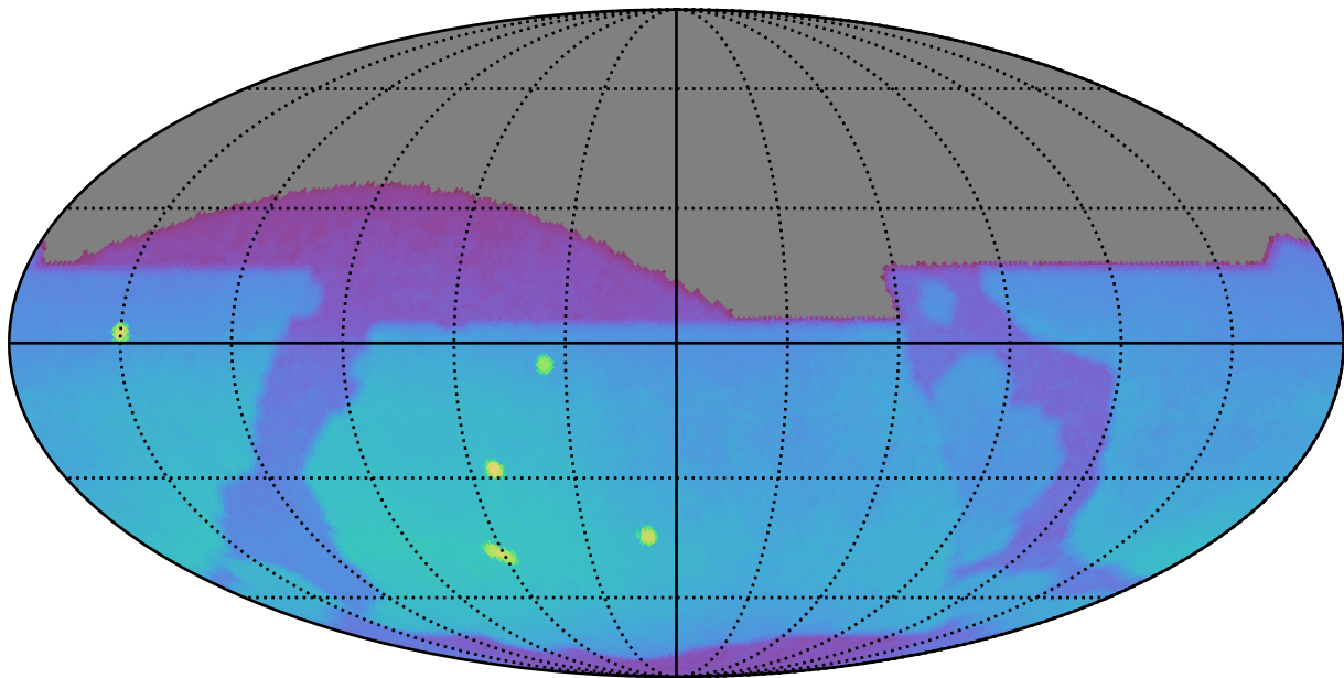
noroll_mjdp0_v3.4_10yrs : Brown Dwarf, L7
