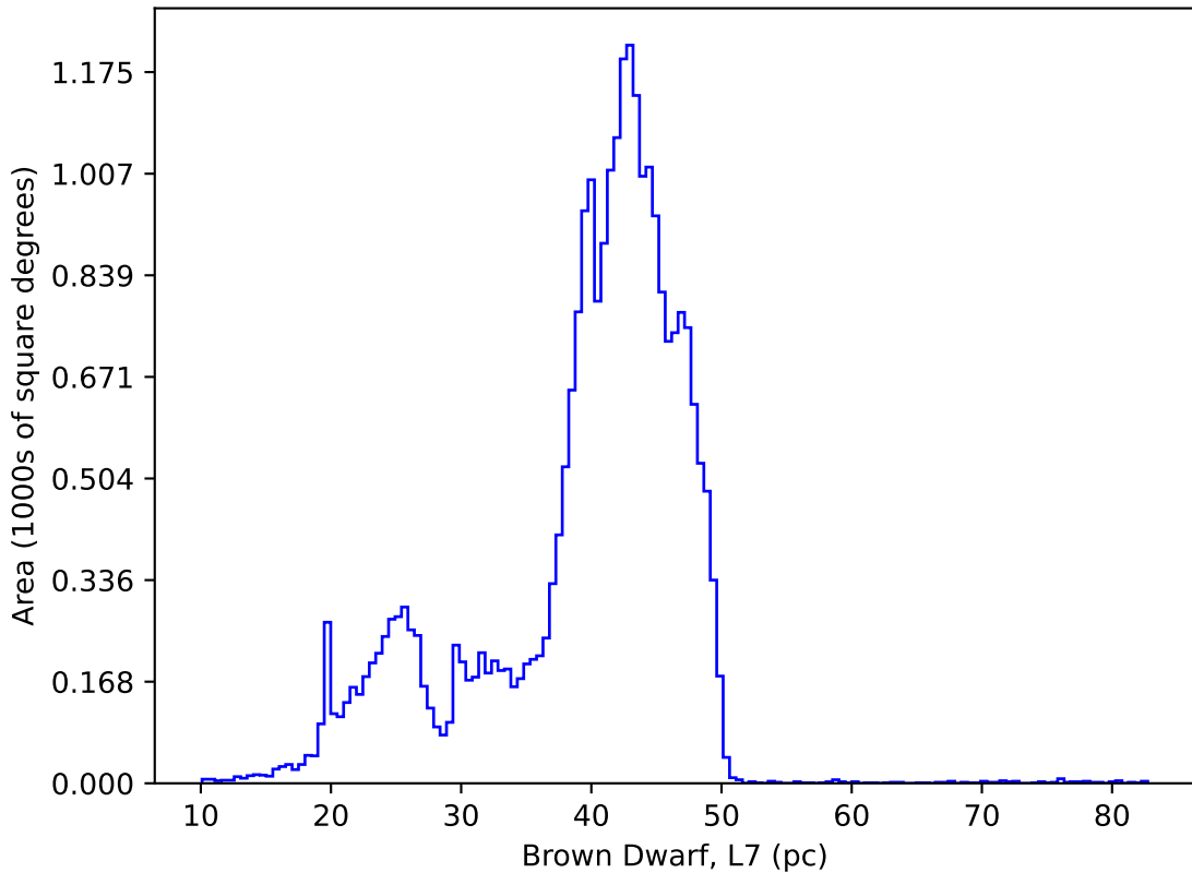
noroll_mjdp0_v3.4_10yrs : Brown Dwarf, L7
