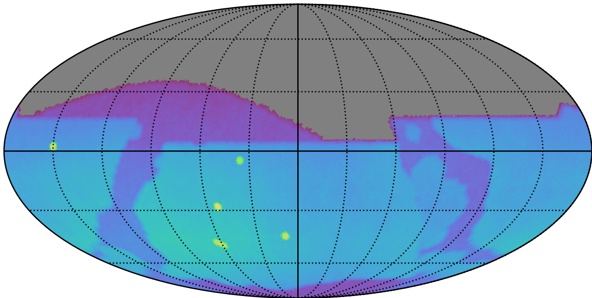
noroll_mjdp0_v3.4_10yrs : Brown Dwarf, L4
