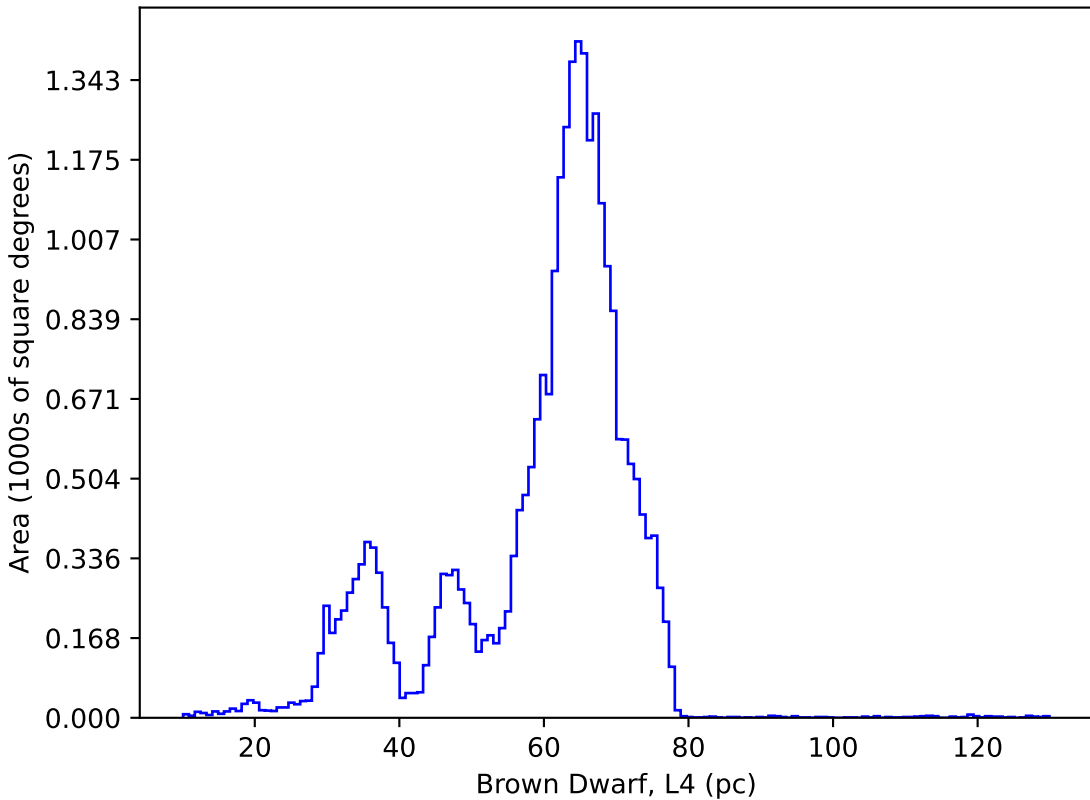
noroll_mjdp0_v3.4_10yrs : Brown Dwarf, L4
