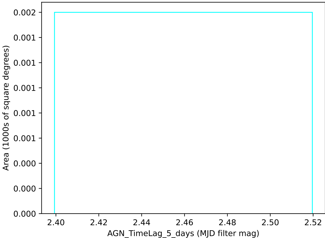
noroll_mjdp0_v3.4_10yrs u band: AGN_TimeLag_5_days
