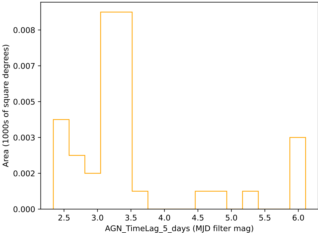
noroll_mjdp0_v3.4_10yrs r band: AGN_TimeLag_5_days
