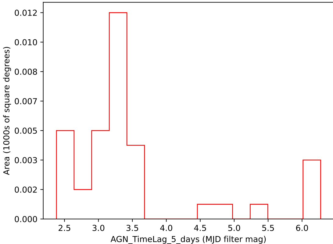
noroll_mjdp0_v3.4_10yrs i band: AGN_TimeLag_5_days
