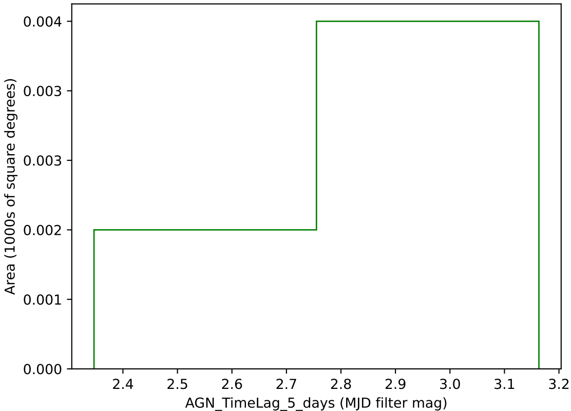
noroll_mjdp0_v3.4_10yrs g band: AGN_TimeLag_5_days
