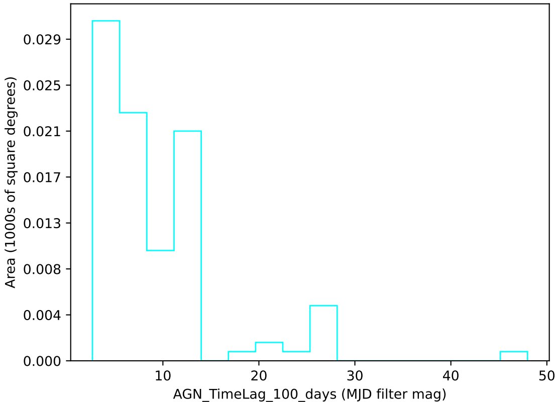
noroll_mjdp0_v3.4_10yrs u band: AGN_TimeLag_100_days
