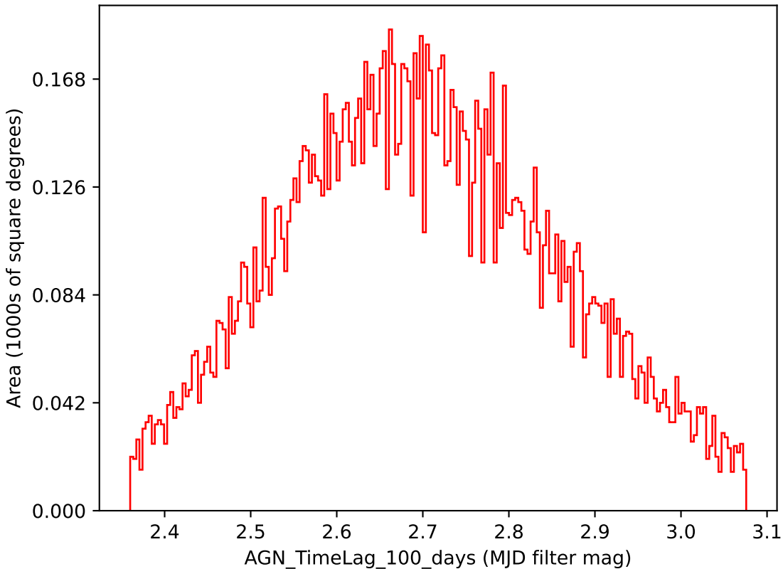
noroll_mjdp0_v3.4_10yrs i band: AGN_TimeLag_100_days
