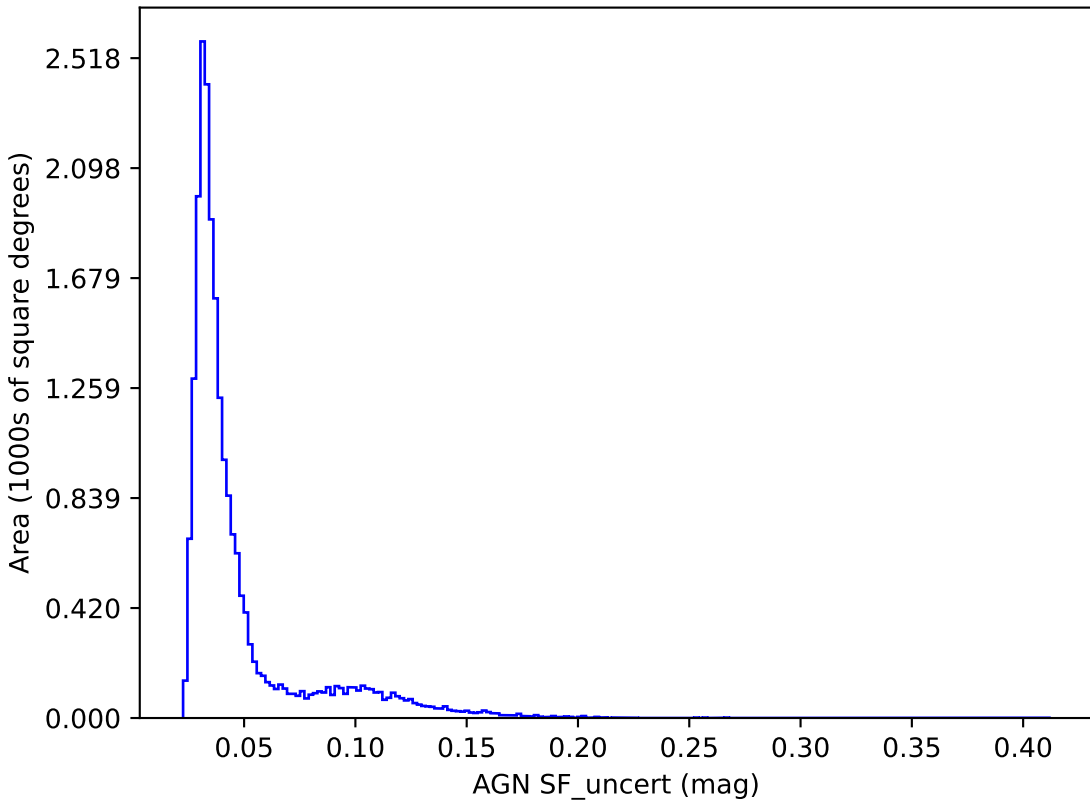
noroll_mjdp0_v3.4_10yrs y band: AGN SF_uncert
