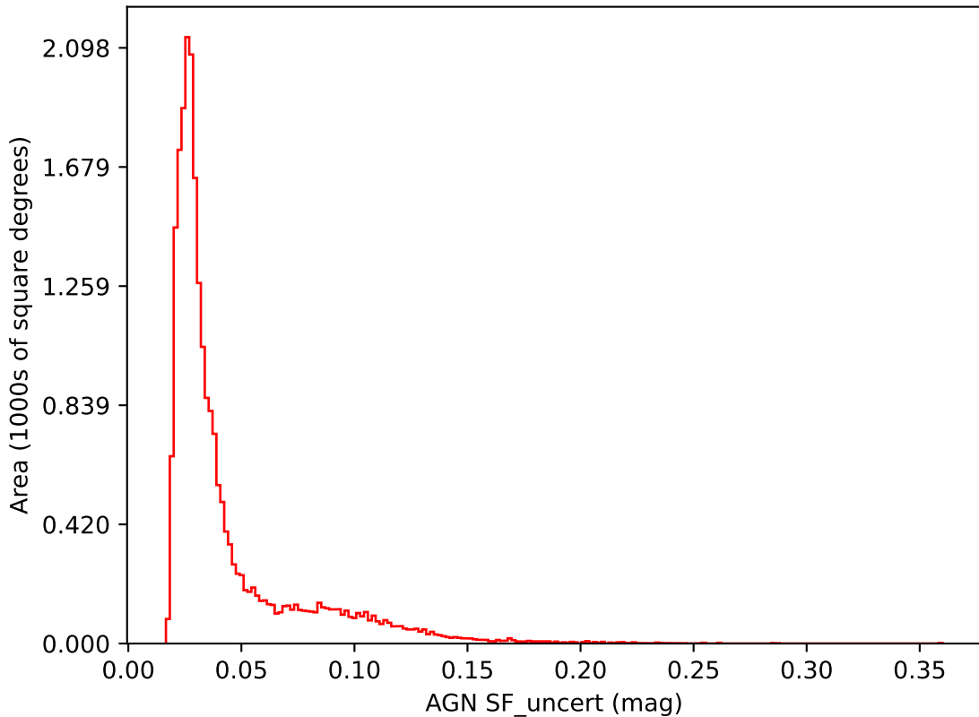
noroll_mjdp0_v3.4_10yrs i band: AGN SF_uncert
